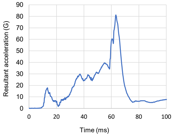
Figure 2 Example of Marginal Head Protection
