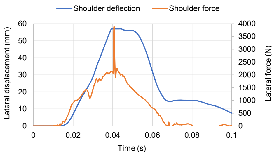
Figure 1 Example of Shoulder Bottoming from Shoulder Deflection and Force Data
